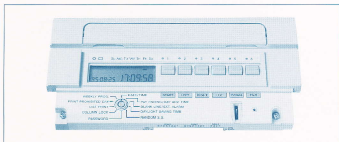
Simple setting and operation with DIP switches and a rotary switch.
